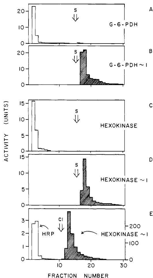
Figure 1. Chromatographic behavior of enzyme-sulfonamide conjugates on a 10-mL column of immobilized carbonic anhydrase ( 0.2 \mu\text{equiv mL}^{-1} ): A, native G-6-PDH; B, G-6-PDH-I; C, native hexokinase; D, hexokinase-I; E, a mixture of hexokinase-I (0.03 mg) and horseradish peroxidase (HRP, 10 mg). Units of G-6-PDH and hexokinase activities are displayed on the left axis; units of HRP activity are displayed on the right axis. Each fraction has a 5-mL volume. The initial eluting buffer in each plot is 0.1 M Tris-phosphate (pH 7.5). At the position indicated by the arrow, the buffer is changed to S, 0.1 M Tris-phosphate (pH 7.5) containing 0.5 M NaCl and 0.01 M p -toluenesulfonamide; Cl, 0.1 M acetate buffer (pH 5.15) containing 1 M NaCl.
